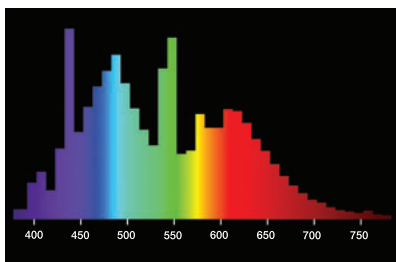
Spectral distribution curve Light colour 965 BIOLUX®
